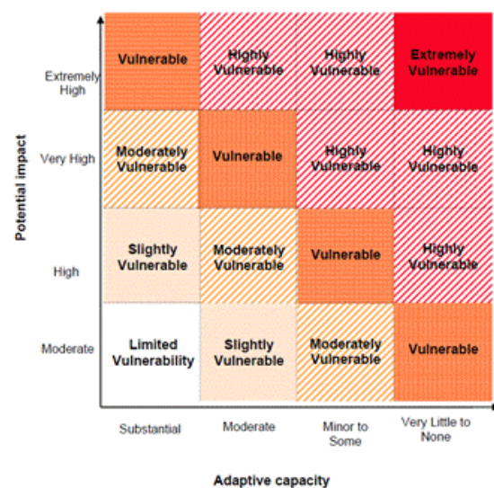
Vulnerability matrix
